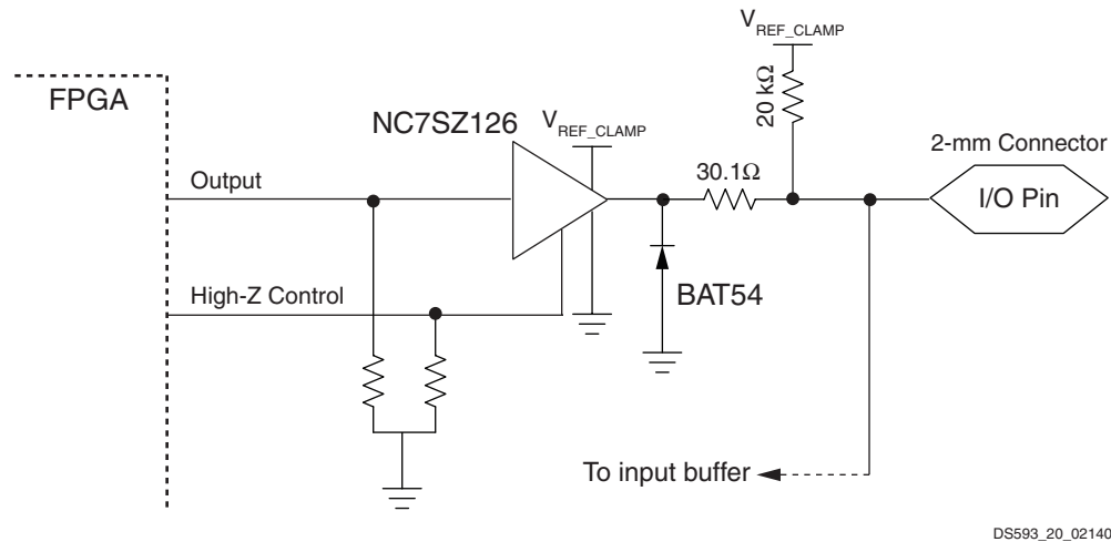
Figure 20: Target Interface Driver Topology
